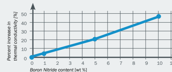
Measured results of the thermal conductivity of HeBoLub® by "flucon fluid control GmbH"
