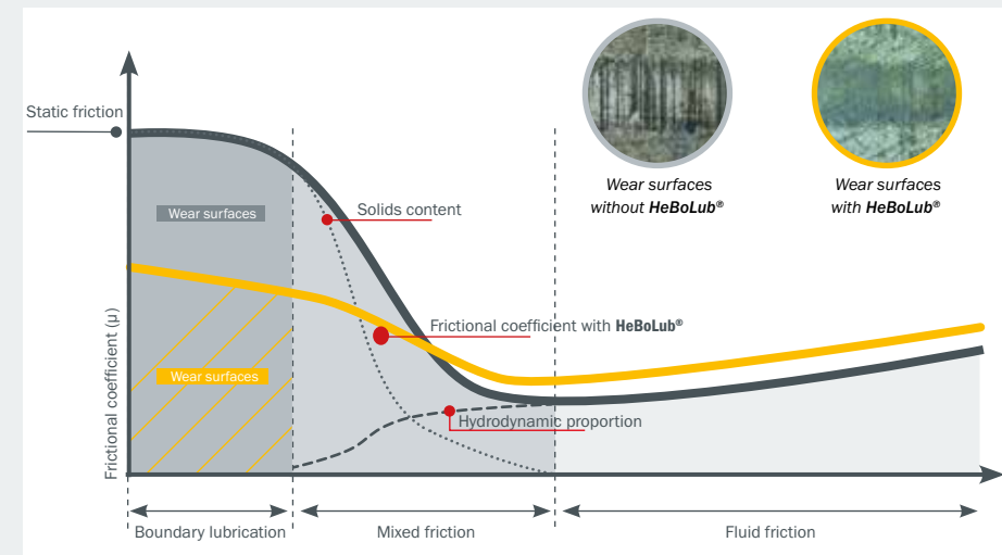
Stribeck-Curve in relation to lubricating parameters Result of a tribological experiment using a cross cylinder tester (XCT) at the Kompetenzzentrum Tribologie, Hochschule Mannheim
