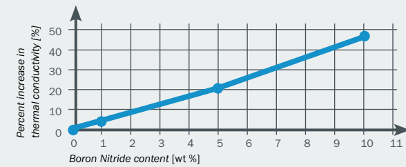
Measured results of the thermal conductivity of HeBoLub® by "flucon fluid control GmbH"
